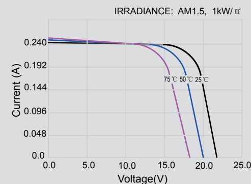
I-V Curves of module SY-M004W at various cell temperatures
