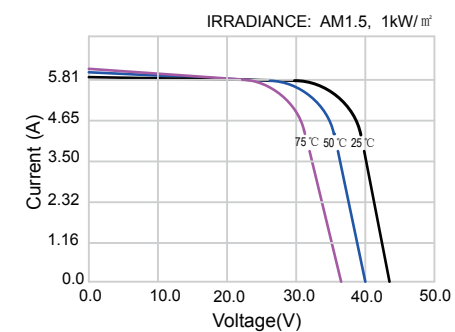
I-V Curves of module SY-M200W at various cell temperatures
