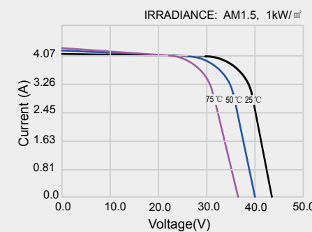
I-V Curves of module SY-M140W at various cell temperatures
