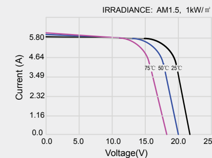
I-V Curves of module SY-M100W at various cell temperatures
