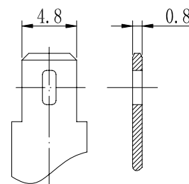
Terminal T1
