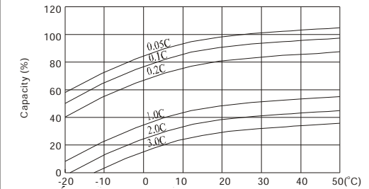
Temperature effects on capacity
