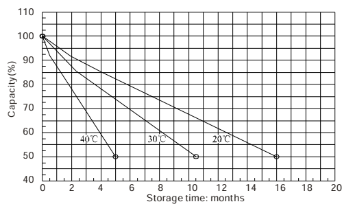
Self-discharge characteristic
